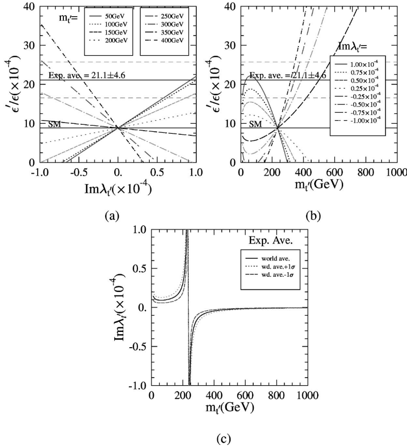
FIG. 2. The diagrams of (a) \epsilon'/\epsilon to \text{Im}\lambda_{t'} , (b) \epsilon'/\epsilon to m_{t'} , and (c) parameter space: \text{Im}\lambda_{t'} to m_{t'} , with B_6^{(1/2)} and B_8^{(3/2)} in lattice gauge theory.
